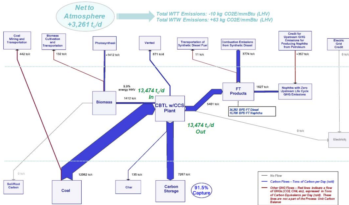
Figure 32: Carbon Flows for 15% Switchgrass (Biomass) by Weight CBTL Plant
